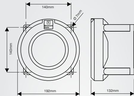
ATEX certified / UL Approved copper free cast aluminium enclosure IP 66
